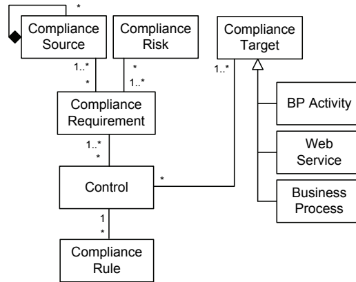
Fig. 5 Excerpt of a Compliance Model
