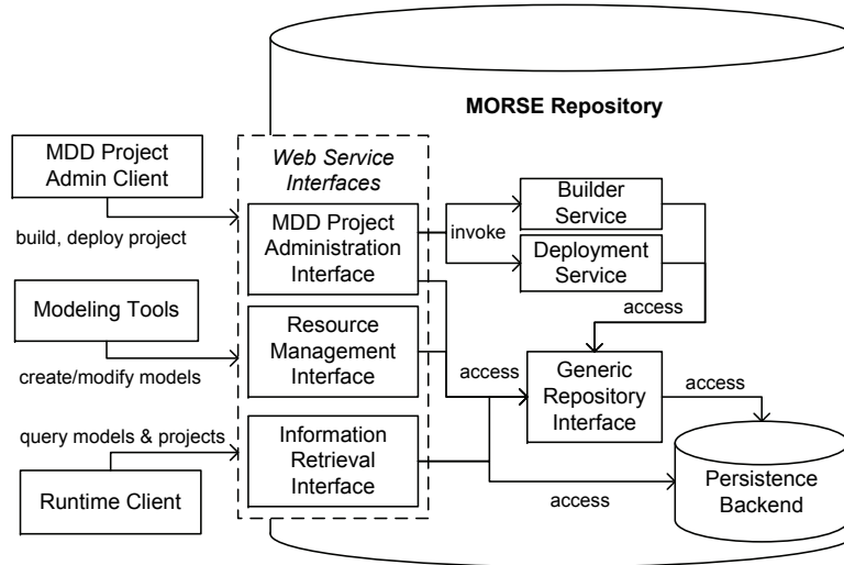
Fig. 2 MORSE Architecture
